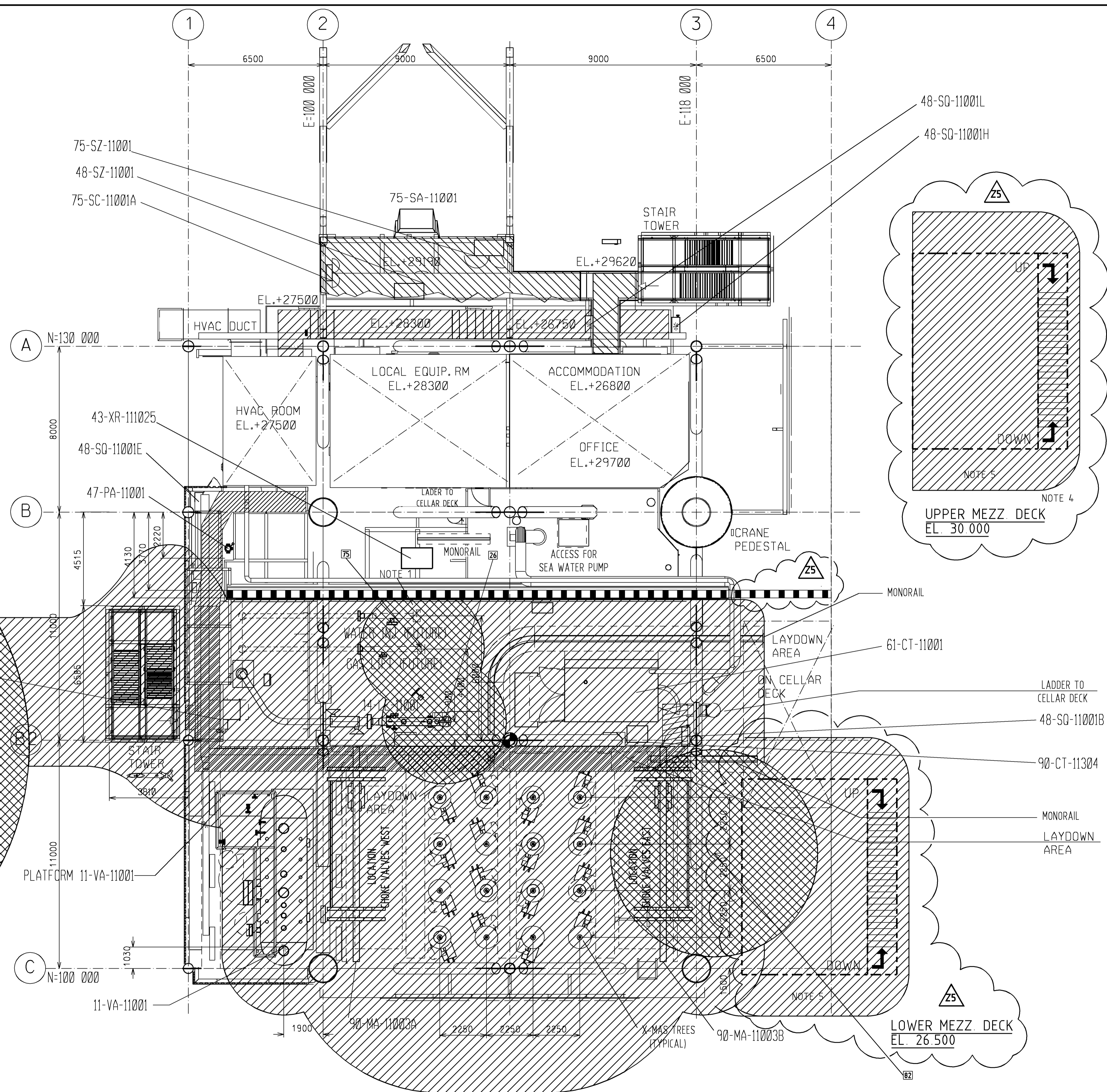
PLAN VIEW MEZZANINE DECK EL. 27.500
