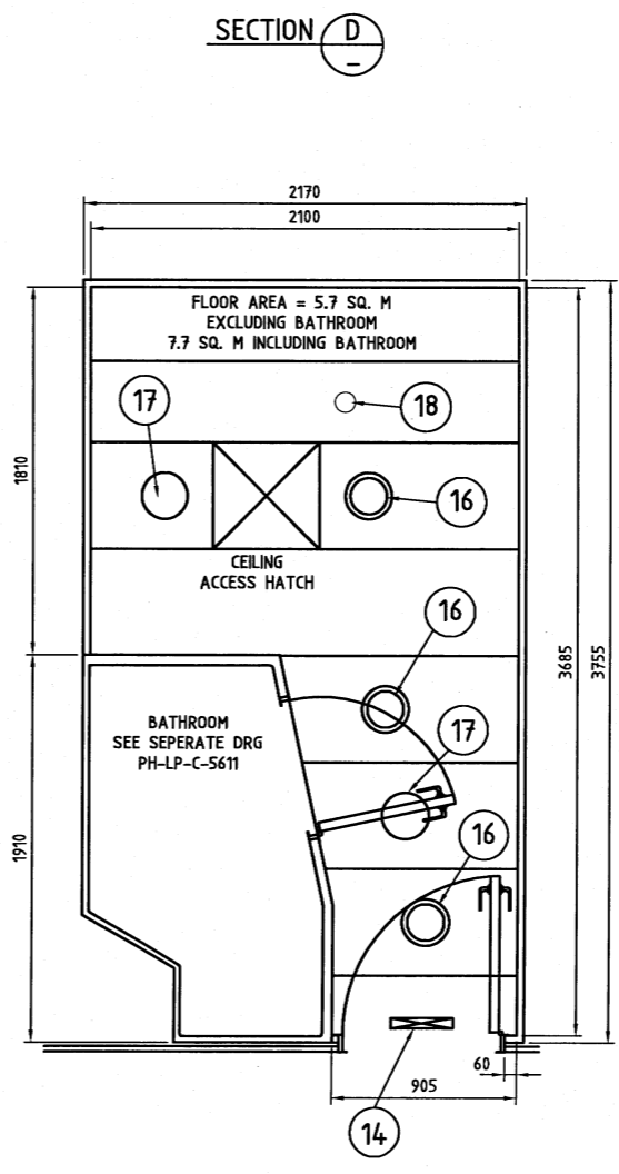
LEFT HAND CABIN TYPICAL 1 PERSON CABIN RIGHT HAND CABIN (SHOWING CABIN CEILING REQUIREMENTS)
