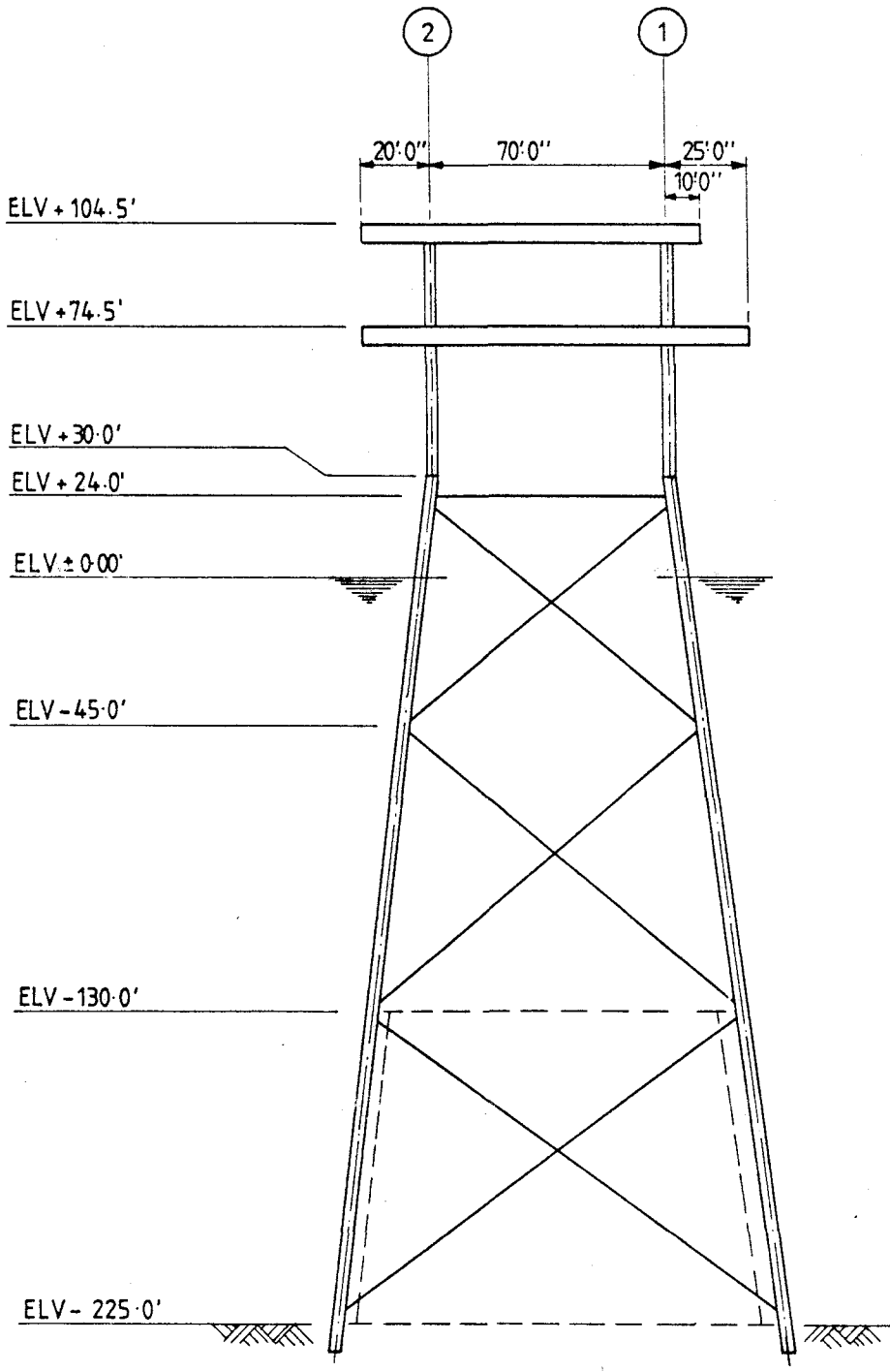
FIG. 2 PLATFORM EAST ELEVATION
