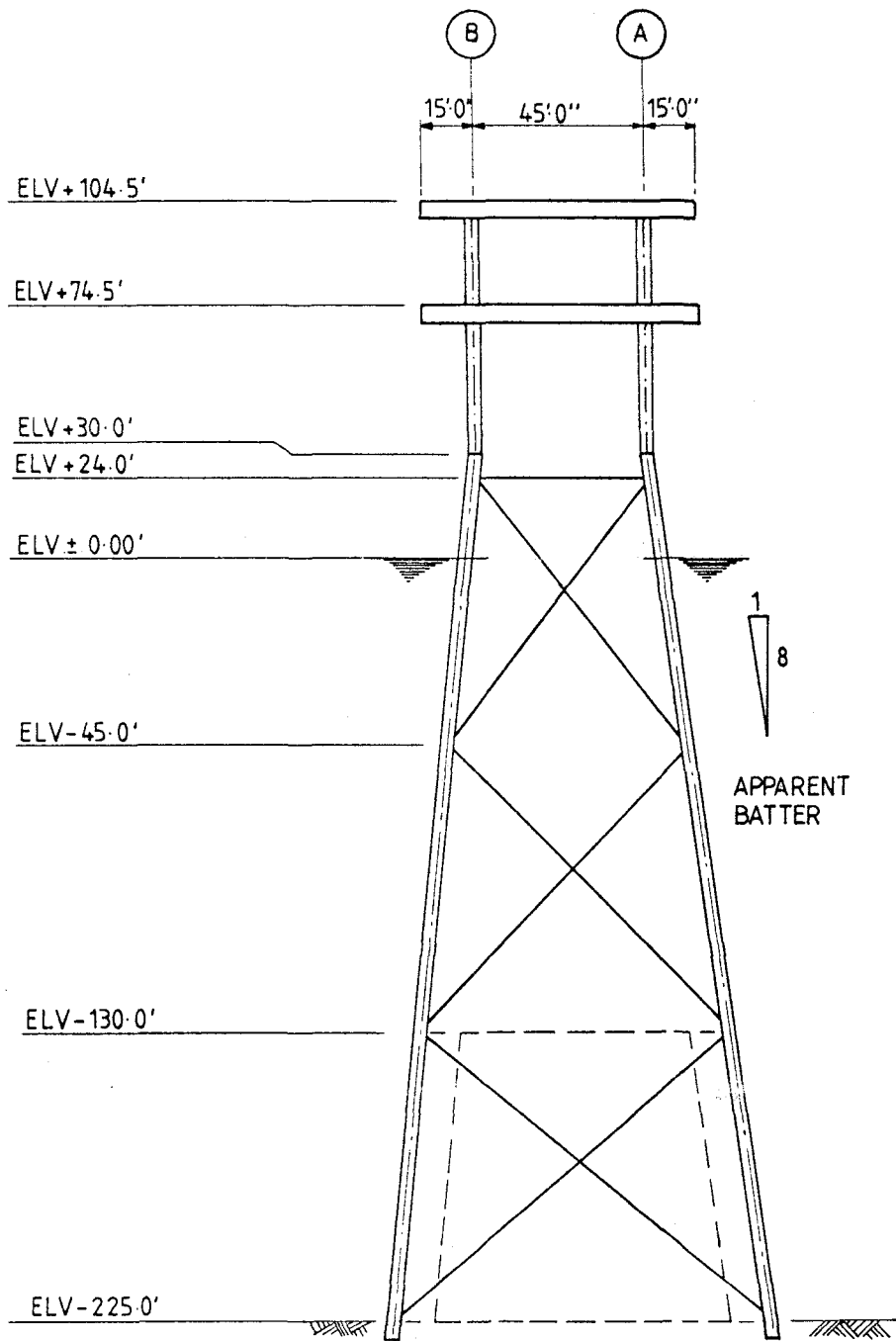
PLATFORM SOUTH ELEVATION
