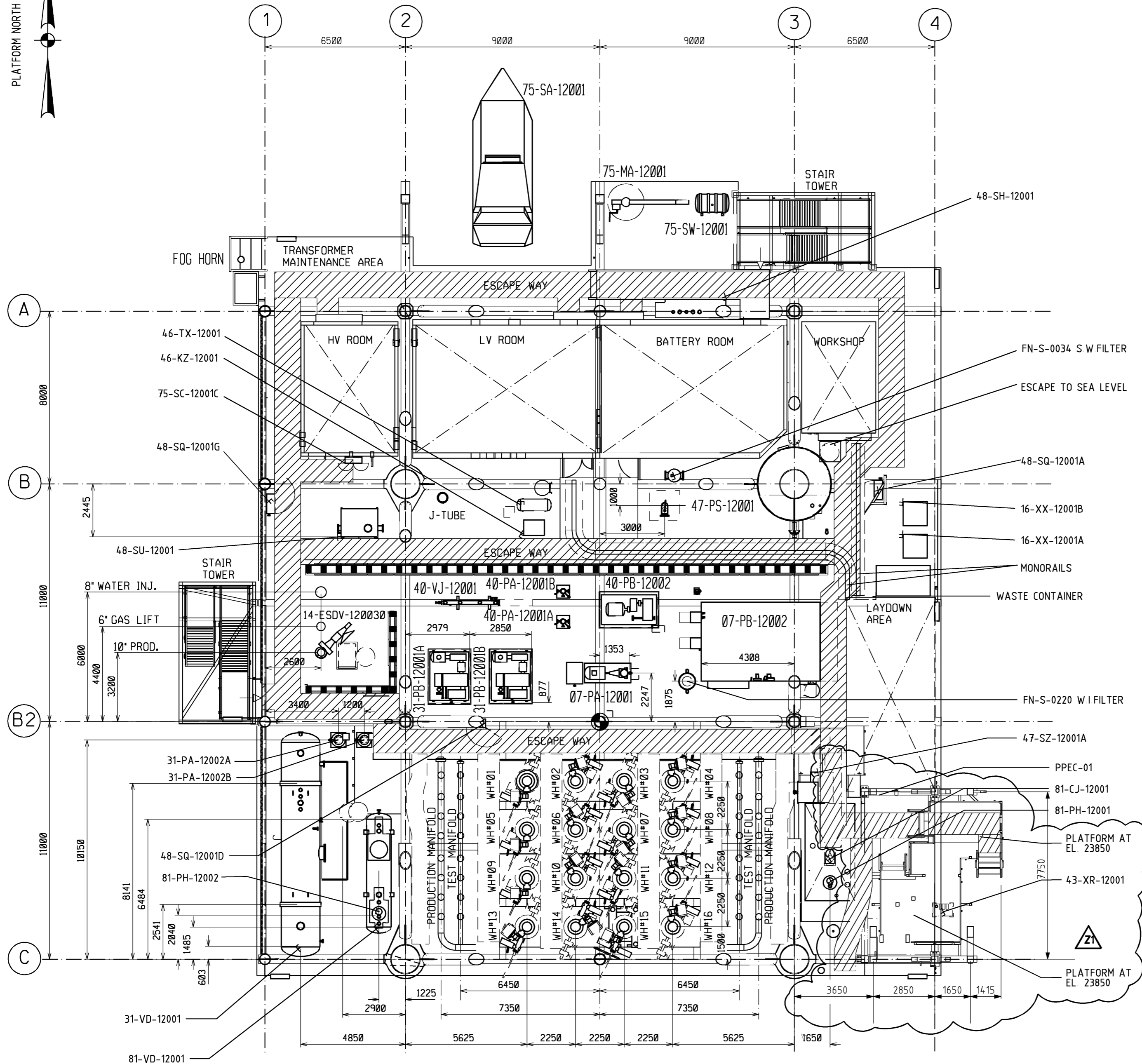
PLAN VIEW CELLAR DECK EL. 23.500
