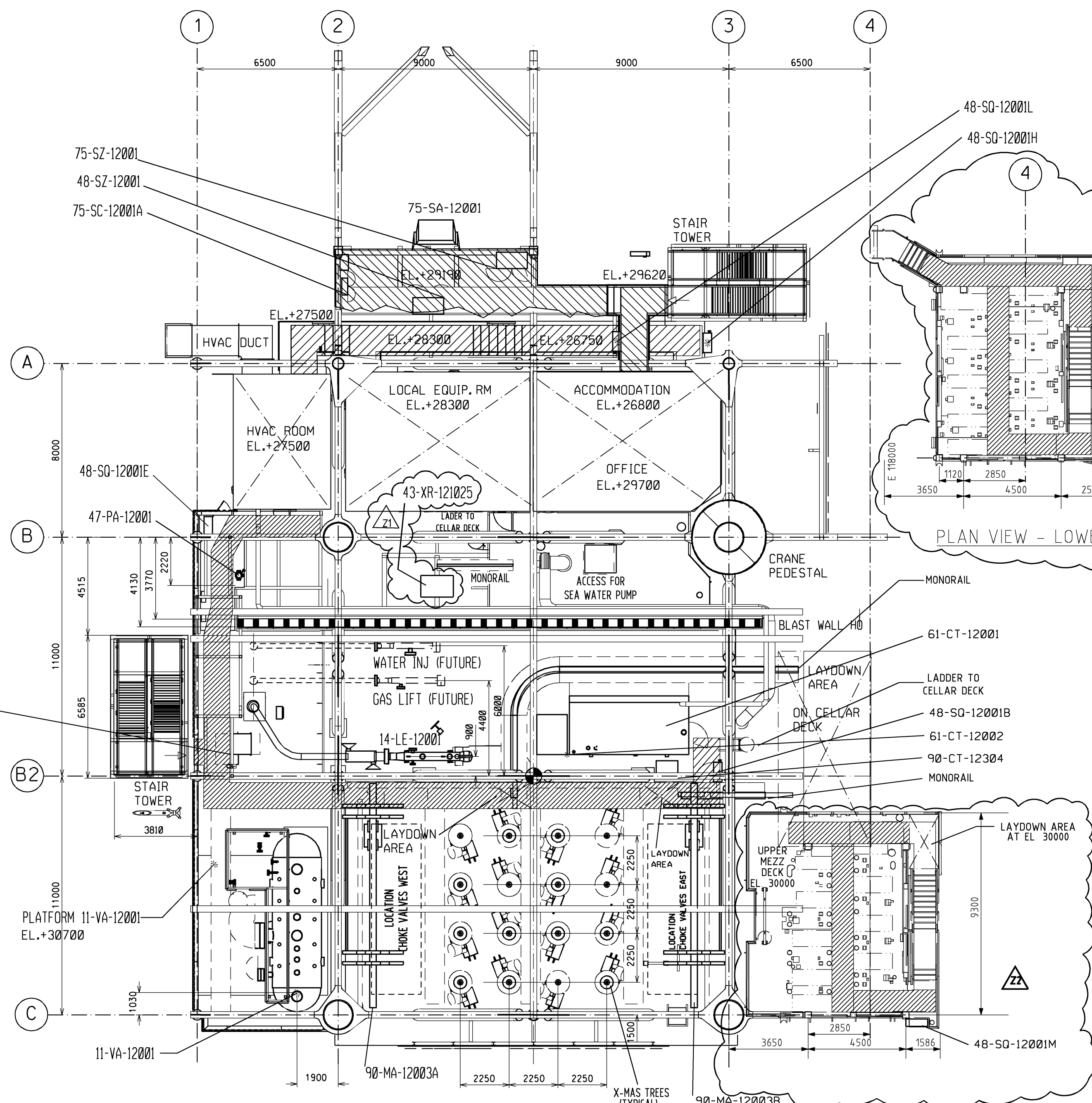
PLAN VIEW MEZZANINE DECK EL. 27 500
