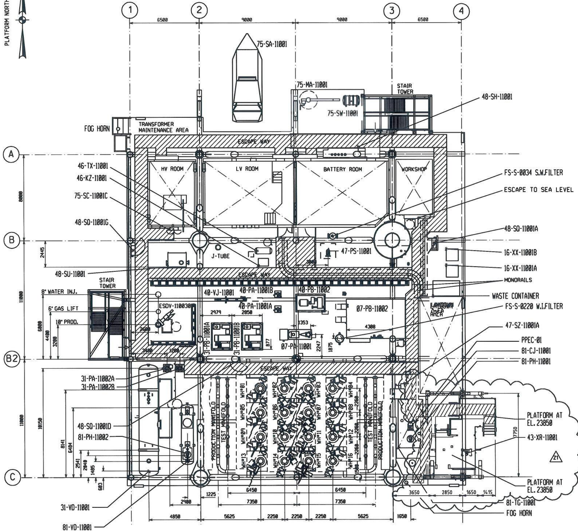
PLAN VIEW CELLAR DECK EL. 23 500
