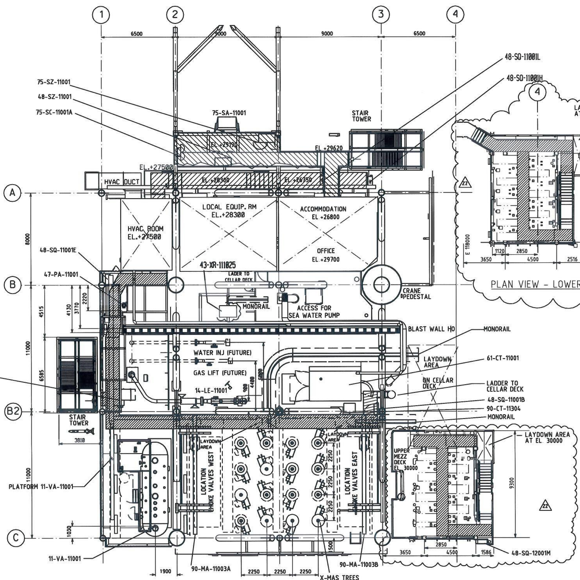
PLAN VIEW MEZZANINE DECK EL. 27.500
